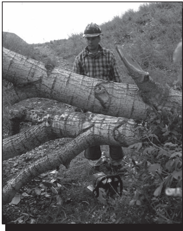
Figure 4-9—Determine the offside. It is the side the log might move to when it is cut.
